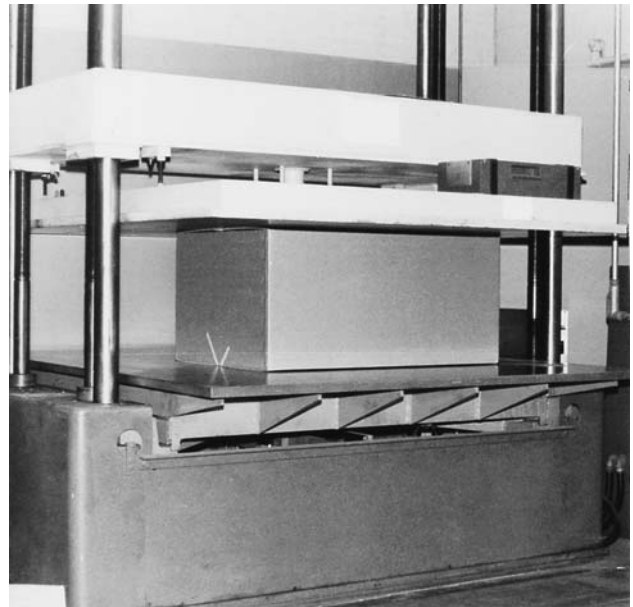
FIG. 2 Compression Applied Top-to-Bottom
